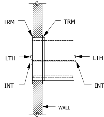
ELEVATION "B"
