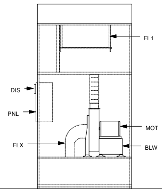
ELEVATION "D" cut away view
