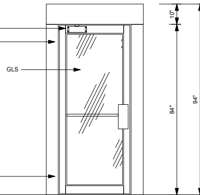
ELEVATION "B"
