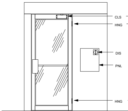
ELEVATION "A"
